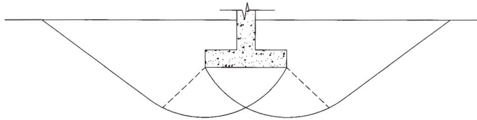
Figure 1. Limit Equilibrium Bearing Capacity of Conventional Spread Footings.
